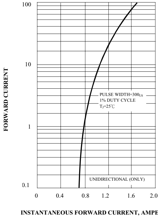
FIG. 11 - INSTANTANEOUS FORWARD VOLTAGE CHARACTERISTICS CURVE
