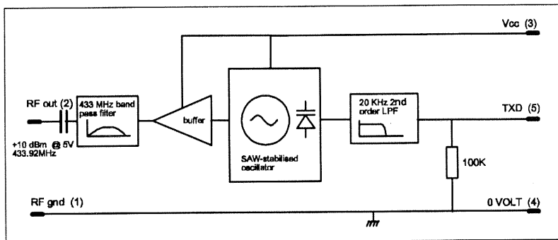
fig. 1: TX2 block diagram
