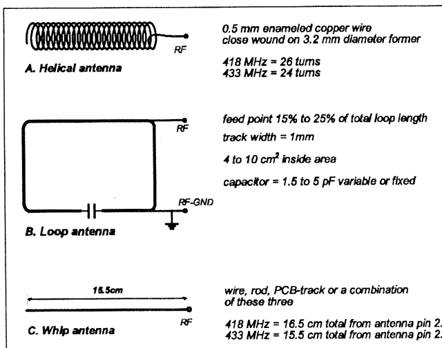
Fig. 8: antenna configurations
