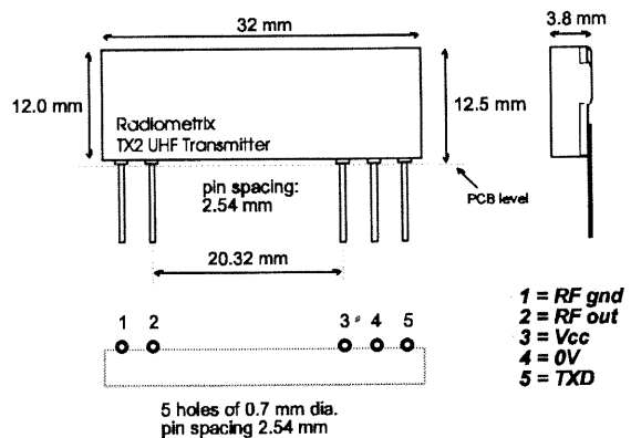
fig. 2: physical dimensions
