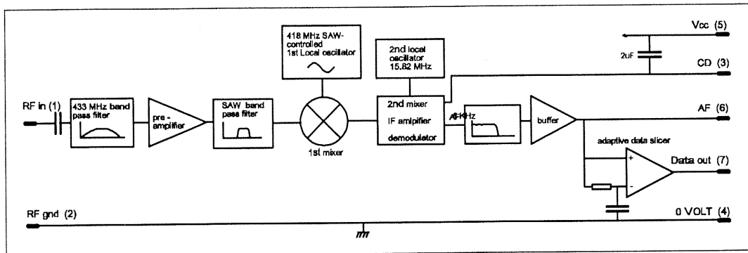
fig. 3: RX2 block diagram
