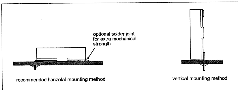
fig. 7: module mounting options
