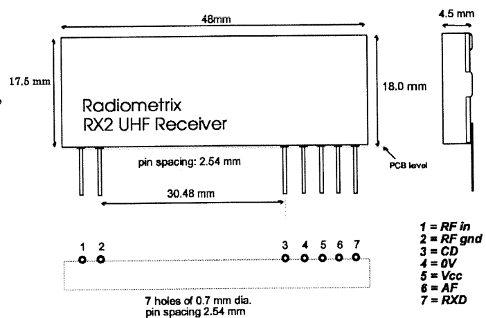
fig. 4: physical dimensions
