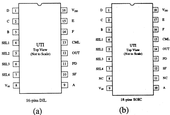
Figure 1 Pin configuration.
