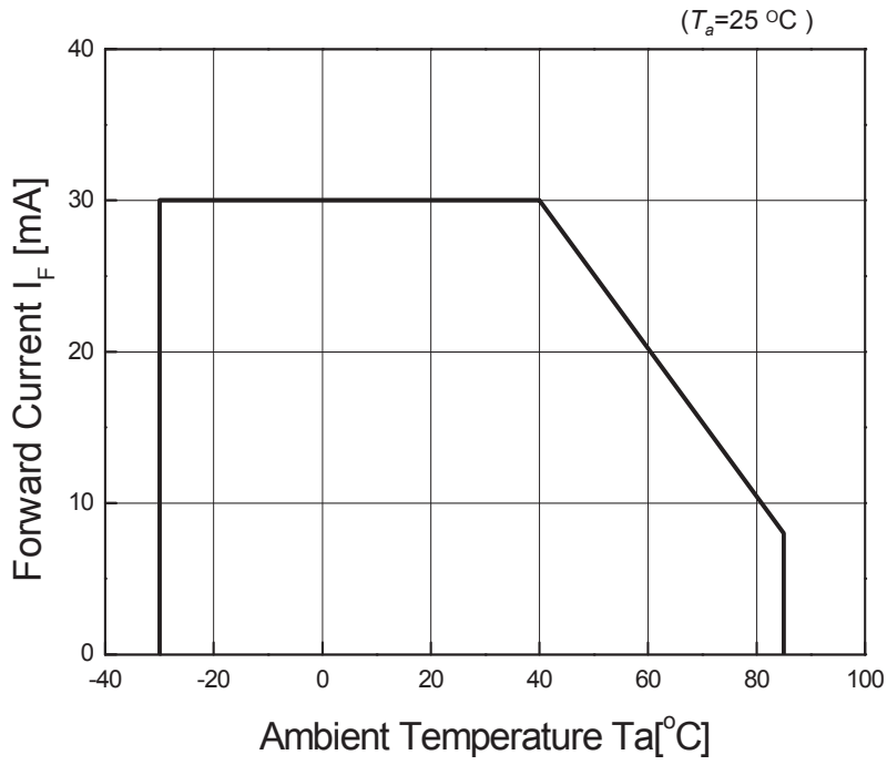
Ambient Temperature vs. Maximum Forward Current
