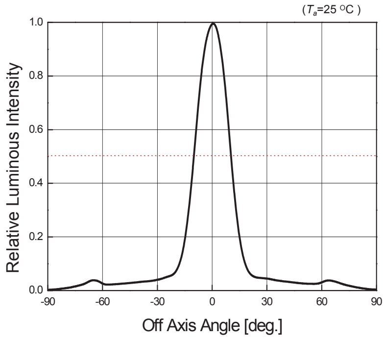
Radiation Diagram
