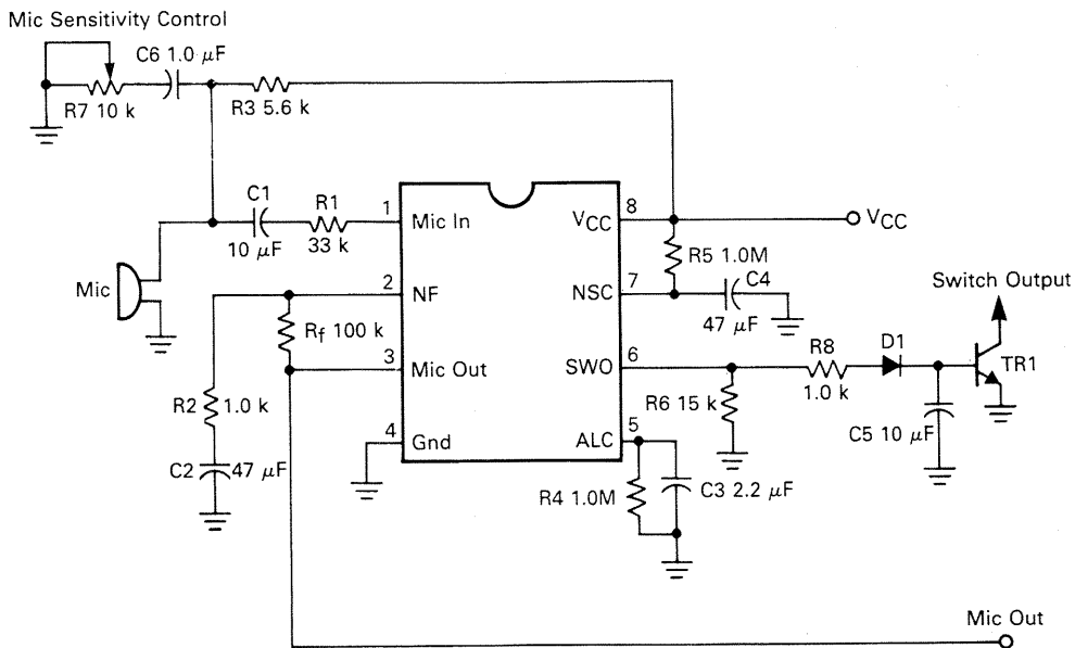
FIGURE 3 — TYPICAL APPLICATION CIRCUIT
