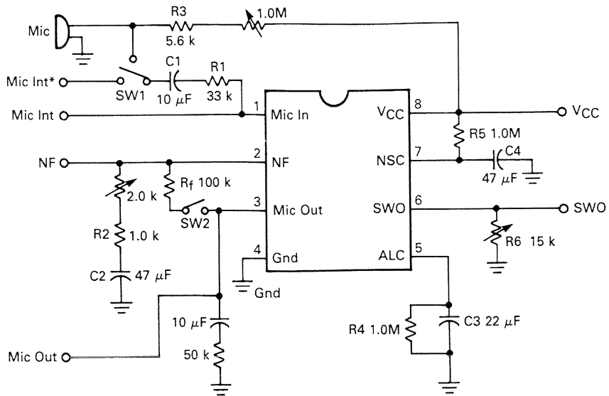
FIGURE 2 — TEST CIRCUIT
