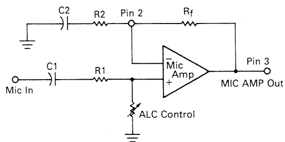
FIGURE 4 — MIC AMPLIFIER WITH ALC
