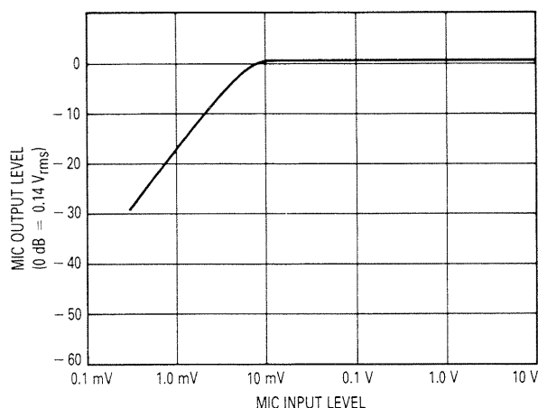
FIGURE 5 — ALC CHARACTERISTICS
