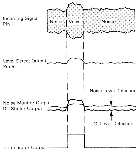
FIGURE 6 — WAVEFORMS OF VOICE DETECTION AND SWITCHING
