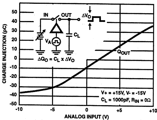
FIGURE 16. CHARGE INJECTION vs ANALOG INPUT
