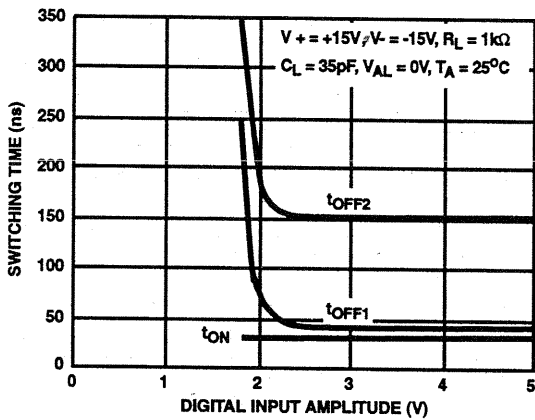
FIGURE 14. SWITCHING TIME vs INPUT LOGIC AMPLITUDE
