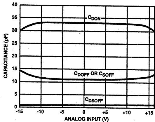
FIGURE 17. CAPACITANCE vs ANALOG INPUT
