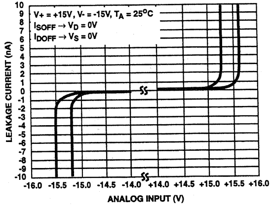
FIGURE 9. LEAKAGE CURRENT vs ANALOG INPUT VOLTAGE
