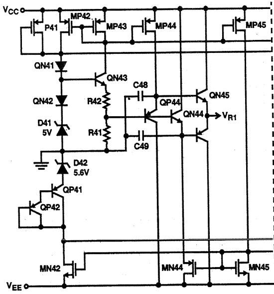
TTL/CMOS REFERENCE CIRCUIT
