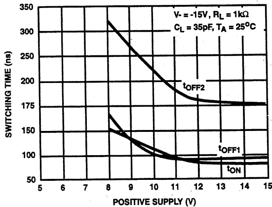
FIGURE 12. SWITCHING TIME vs POSITIVE SUPPLY VOLTAGE
