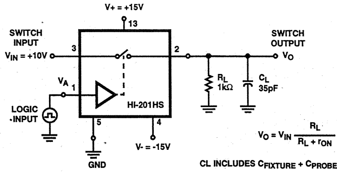
FIGURE 20. SWITCHING TEST CIRCUIT ( t_{ON} , t_{OFF1} , t_{OFF2} )
