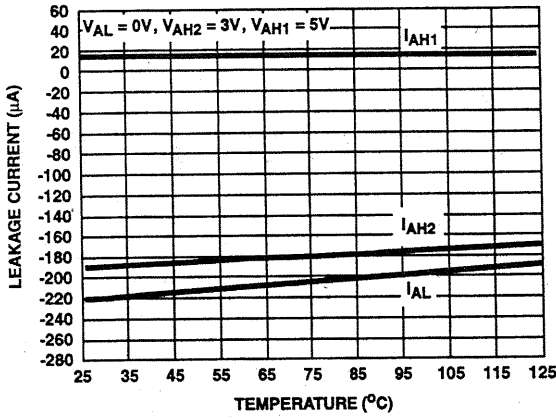
FIGURE 8. DIGITAL INPUT LEAKAGE CURRENT vs TEMPERATURE†
