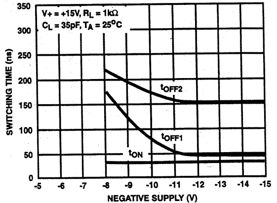
FIGURE 13. SWITCHING TIME vs NEGATIVE SUPPLY VOLTAGE
