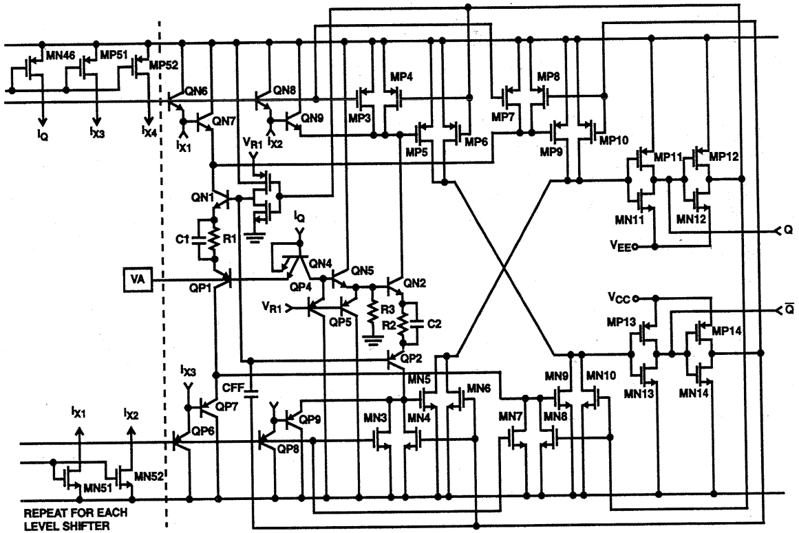
DIGITAL INPUT BUFFER AND LEVEL SHIFTER
