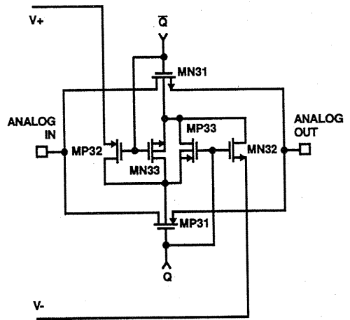
SWITCH CELL
