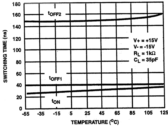
FIGURE 10. SWITCHING TIME vs TEMPERATURE
