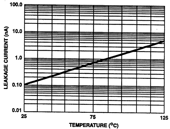
FIGURE 5. I_{D(ON)} vs TEMPERATURE†
