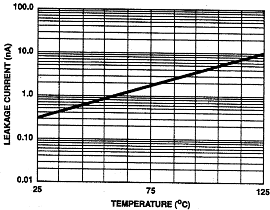
FIGURE 4. I_{S(OFF)} OR I_{D(OFF)} vs TEMPERATURE†
