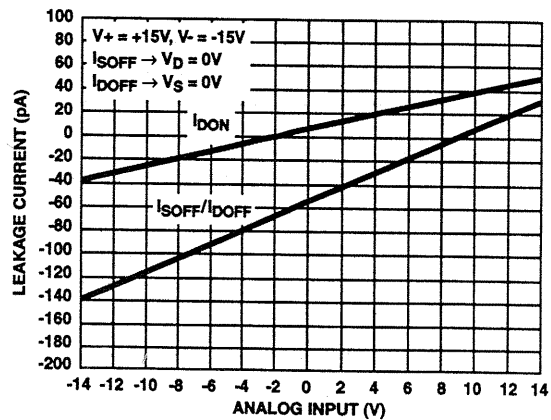
FIGURE 7. LEAKAGE CURRENT vs ANALOG INPUT VOLTAGE
