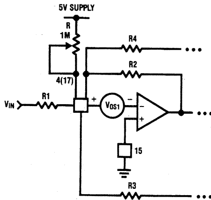
FIGURE 20. Method for Trimming V_{OS}
