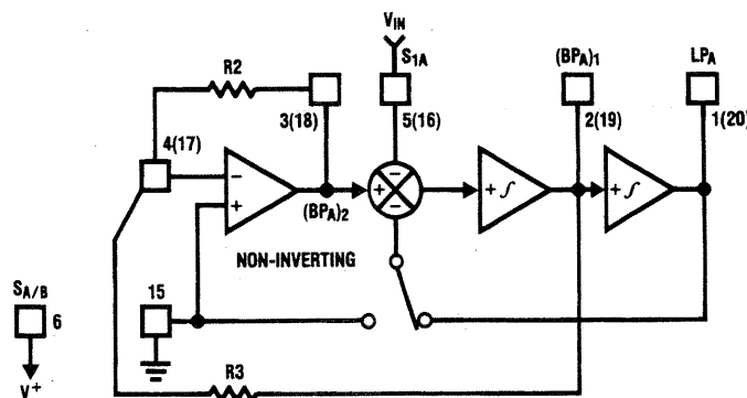
FIGURE 8. MODE 1a
