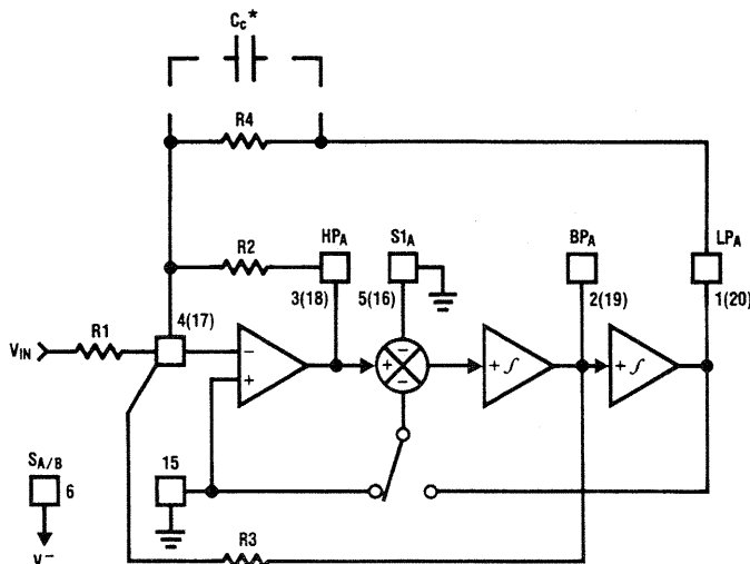
FIGURE 10. MODE 3
