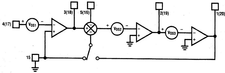
FIGURE 19. MF10 Offset Voltage Sources
