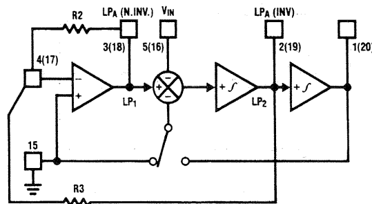
FIGURE 15. MODE 6b
