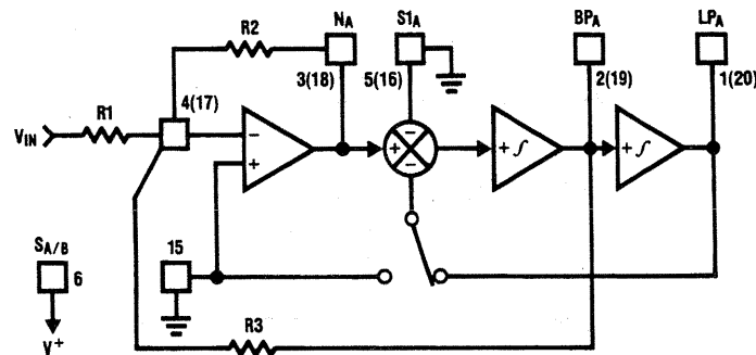
FIGURE 7. MODE 1
