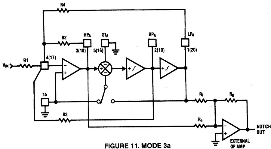
FIGURE 11. MODE 3a
