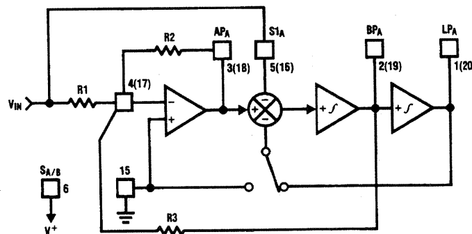
FIGURE 12. MODE 4
