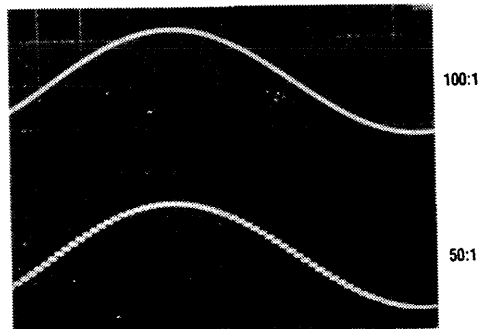
FIGURE 21. The Sampled-Data Output Waveform
