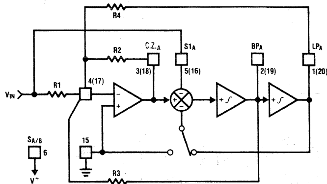
FIGURE 13. MODE 5
