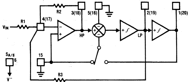
FIGURE 14. MODE 6a
