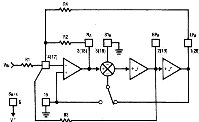
FIGURE 9. MODE 2
